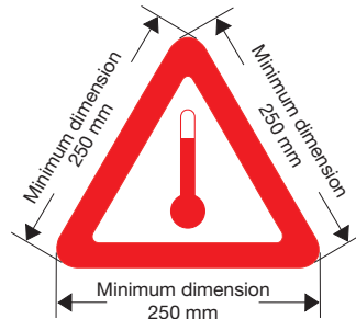
Mark for transport at elevated temperature
