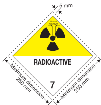
Placard for radioactive material of class 7
