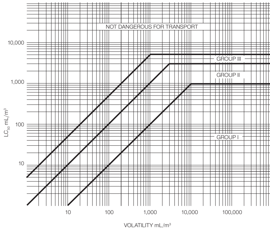
Figure 2-3 – Inhalation toxicity: packing group borderlines
