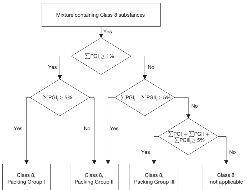
Figure 2.8.4.3 – Calculation method
