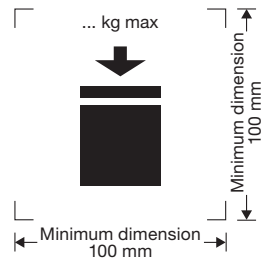
IBC's capable of being stacked
