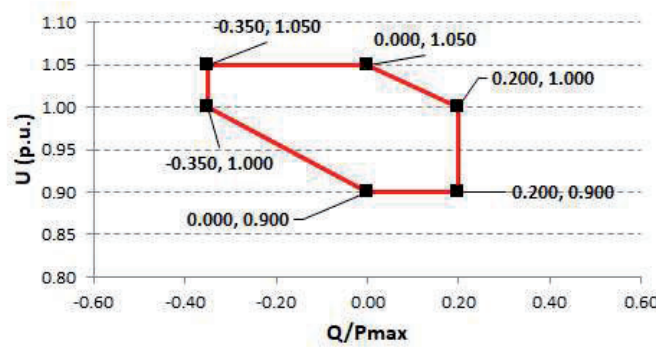
Figure 2: U-Q/Pmax-profile of ESMs connected at 400kV
