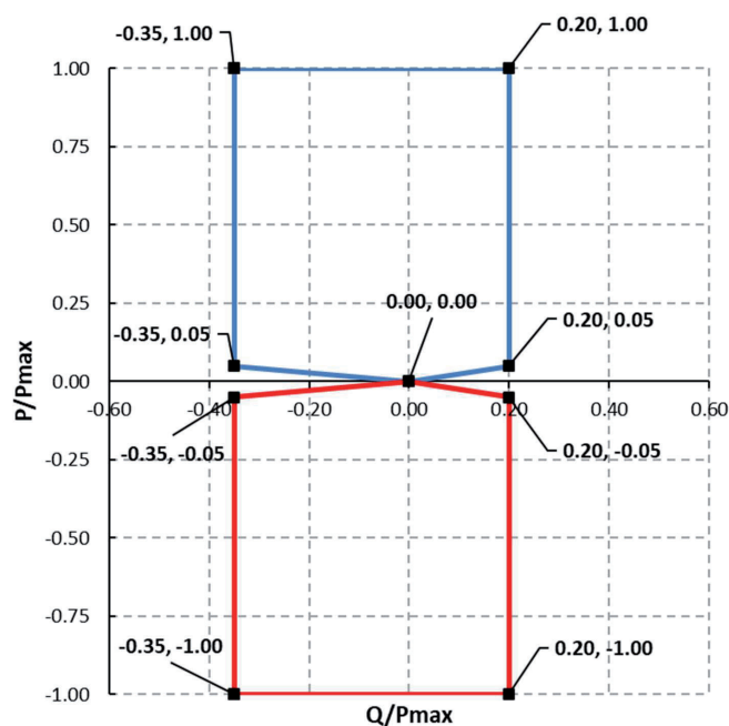
Figure 3: P-Q/Pmax-profile of ESMs connected at 150/400kV
